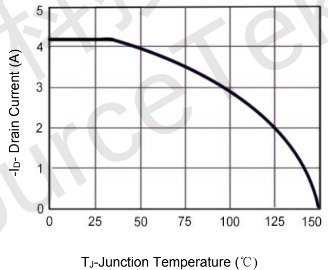
Figure 4 Drain Current
