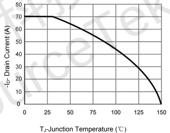
Figure 4 Drain Current
