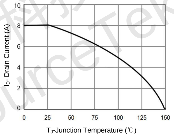
Figure 4 Drain Current
