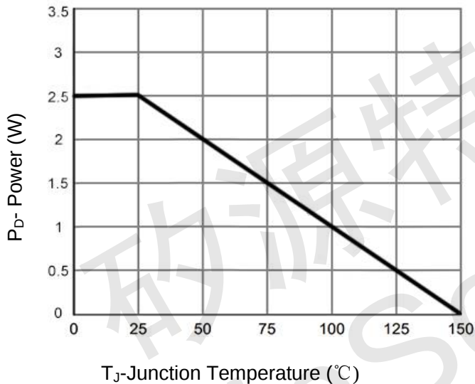
Figure 3 Power De-rating
