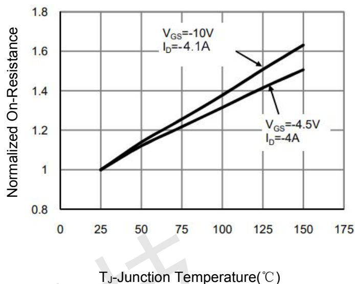
TJ-Junction Temperature(°C) Figure 8 Rdson vs Junction Temperature
