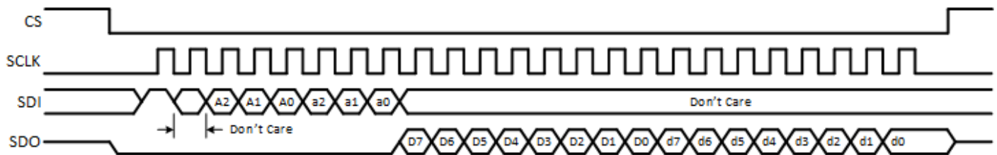
Figure 9 • SPI Read Command
