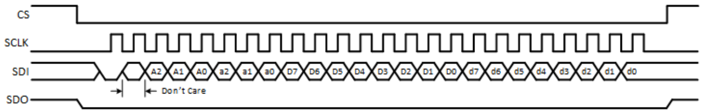
Figure 8 • SPI Write Command
