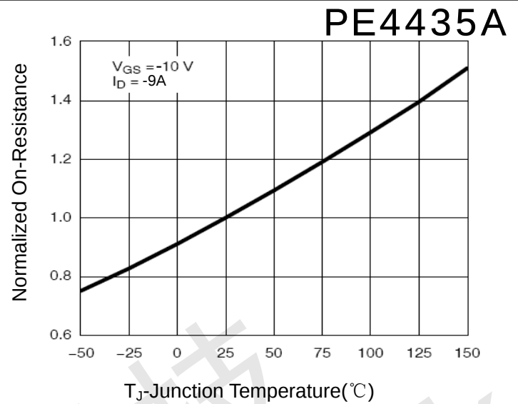
Figure 8 Drain-Source On-Resistance
