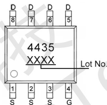
Marking and pin Assignment
