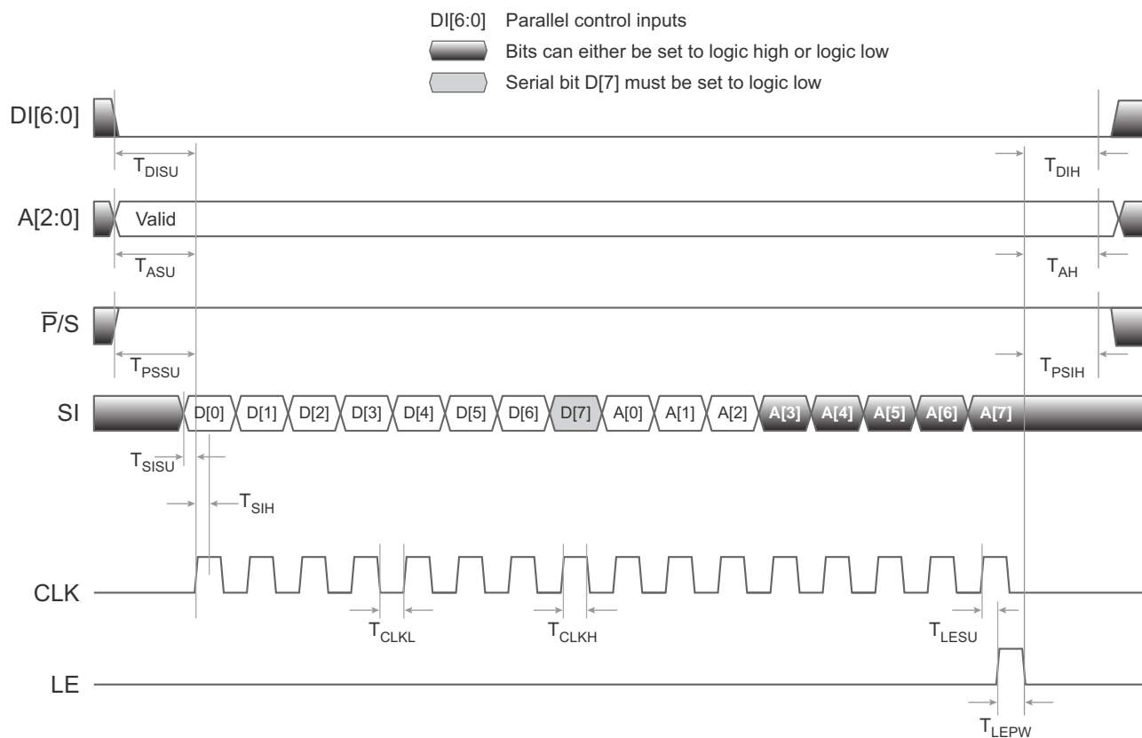
Figure 3 • Serial Addressable Timing Diagram
