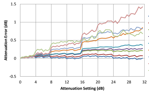
Figure 13. 0.5 dB Attenuation Error vs. Frequency
