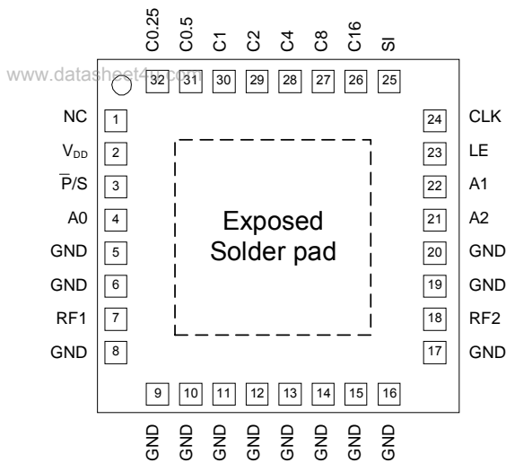
Figure 18. Pin Configuration (Top View)
