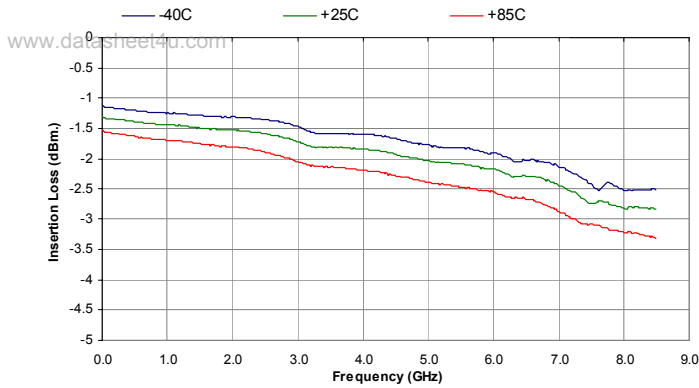
Figure 7. Insertion Loss vs. Temperature
