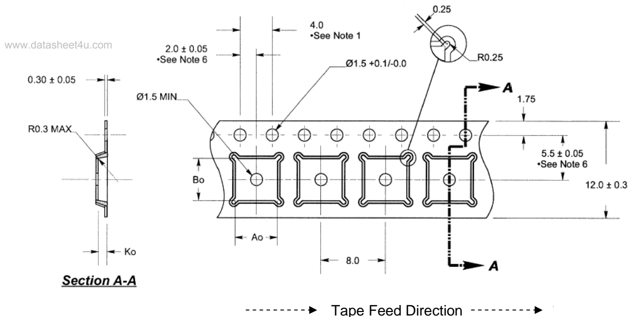
Figure 25. Tape and Reel Drawing
