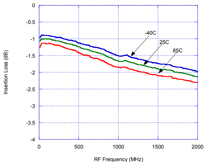
Figure 6. Insertion Loss ( Z_o = 75\ \text{ohms} )
