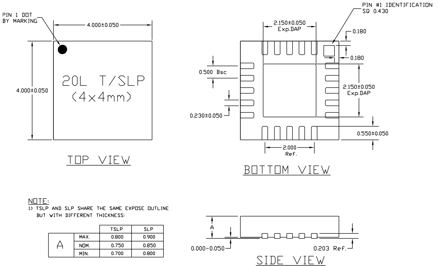
Figure 20. Package Drawing
