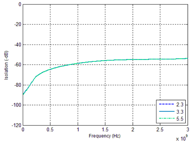
Figure 18. Isolation vs. V_{DD} (RFC-RFX)
