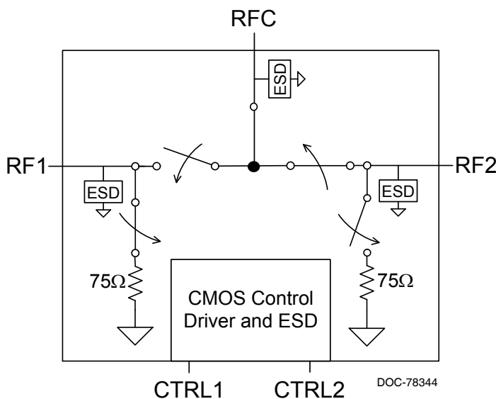
Figure 1. Functional Diagram
