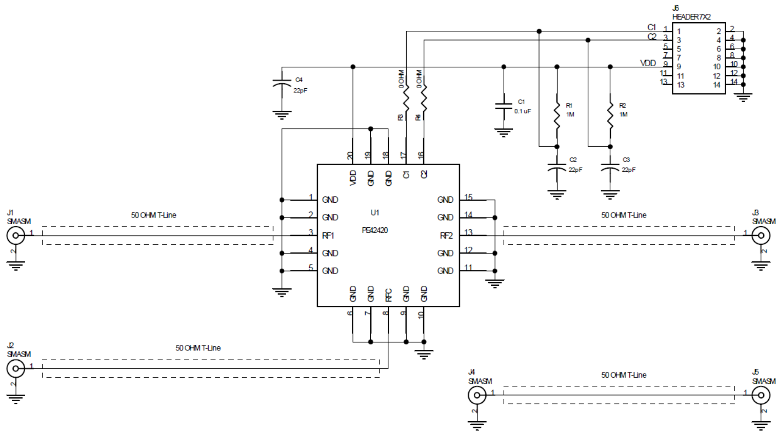
Figure 18. Evaluation board schematic
