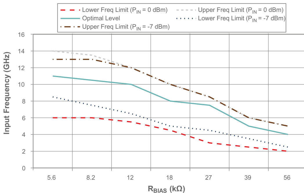
Figure 3 • Frequency vs R_{BIAS}
