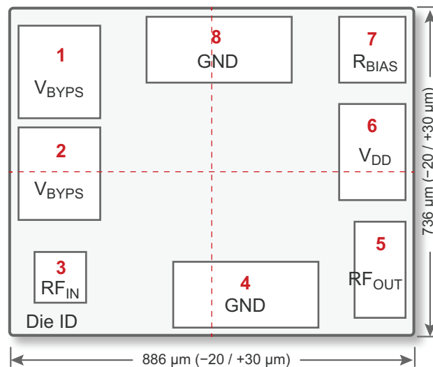
Figure 13 • Pad Layout for PE35400 (1)(2)
