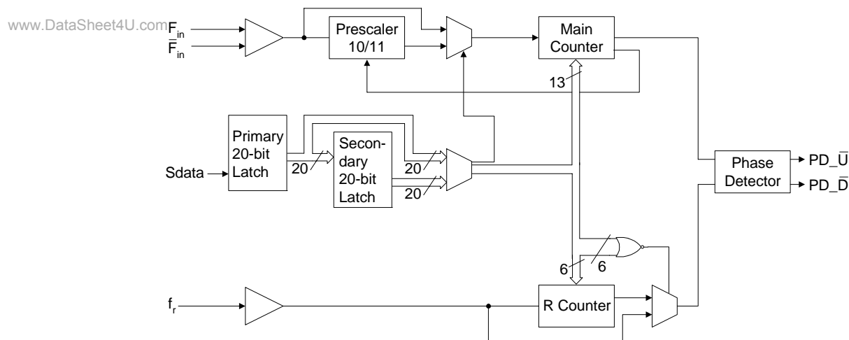
Figure 1. Block Diagram
