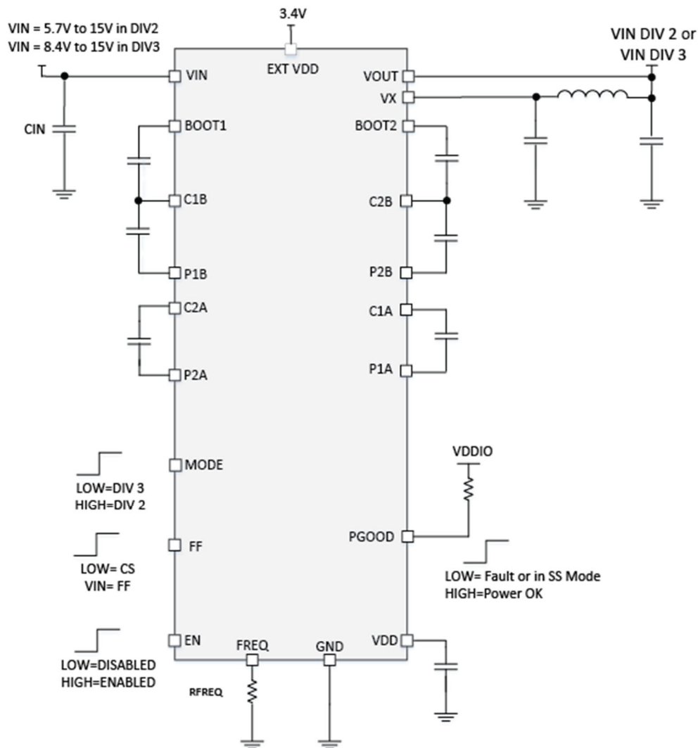
Figure 5. Simplified Application Circuit
