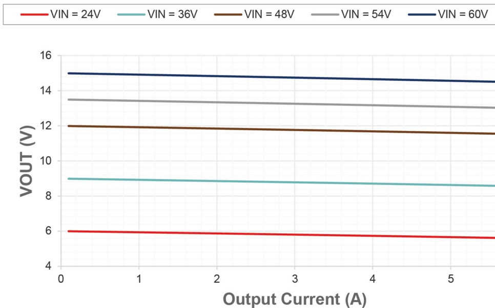
Figure 8. V_{OUT} vs. load current, V_{IN} = 24, 36, 48, 54, 60V , T_A = 25\text{ }^{\circ}C
