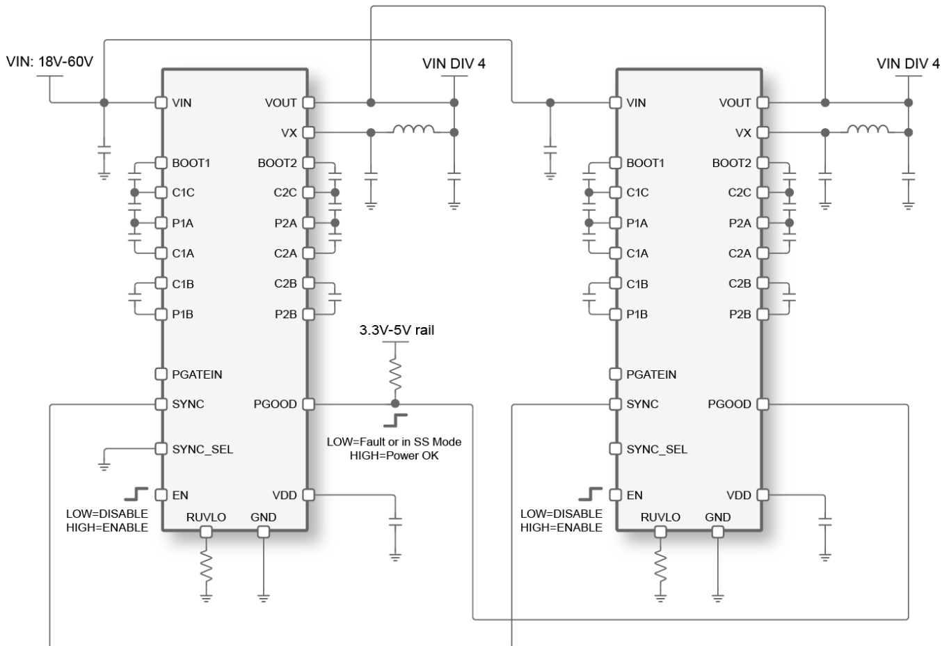
Figure 31. PE25204 Parallel Operation
