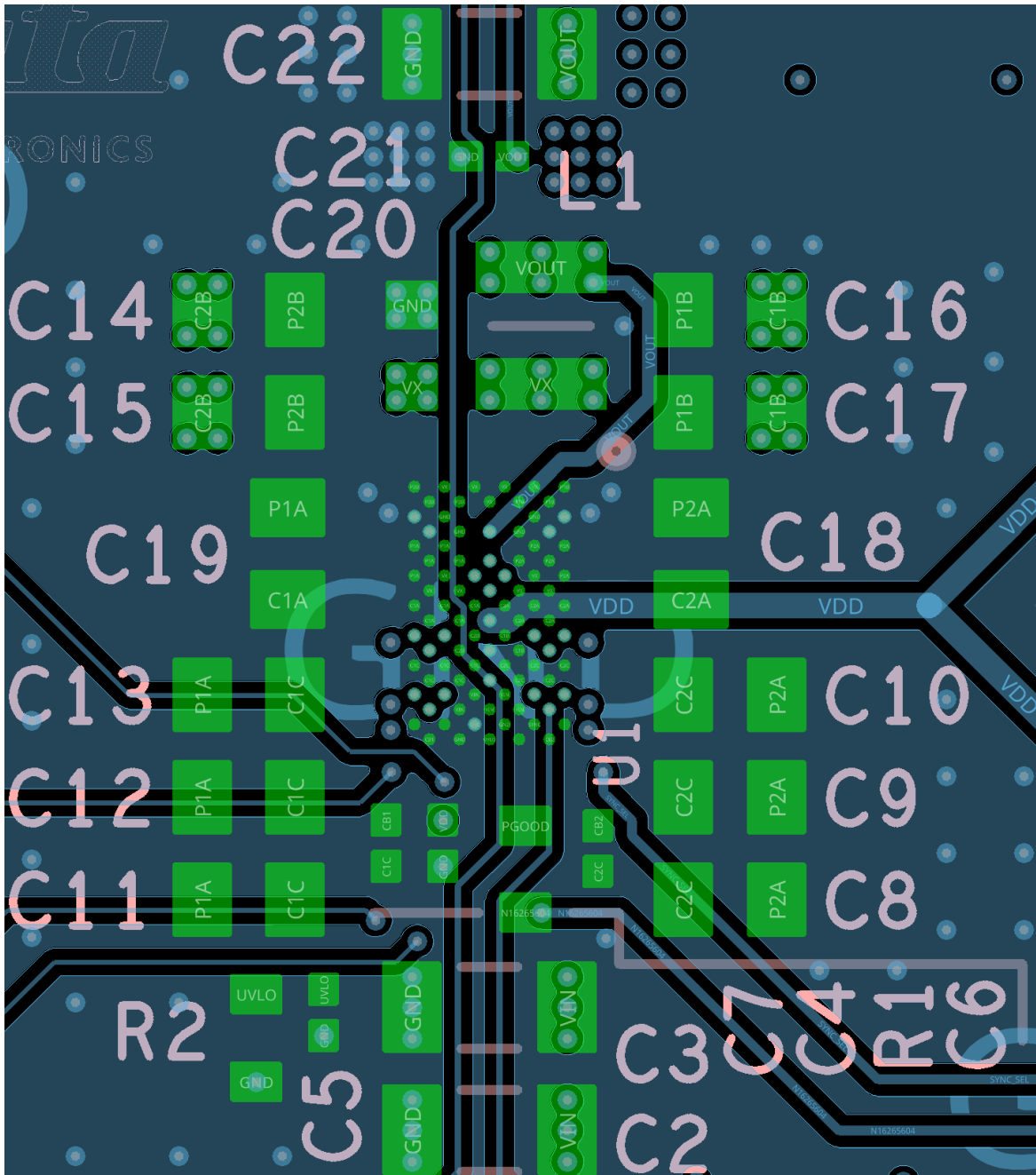
Figure 29. Inner Layer 2
