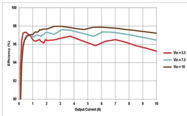
Figure 7. Efficiency vs. Load Current Cycle Skipping, DIV2, 25 °C
