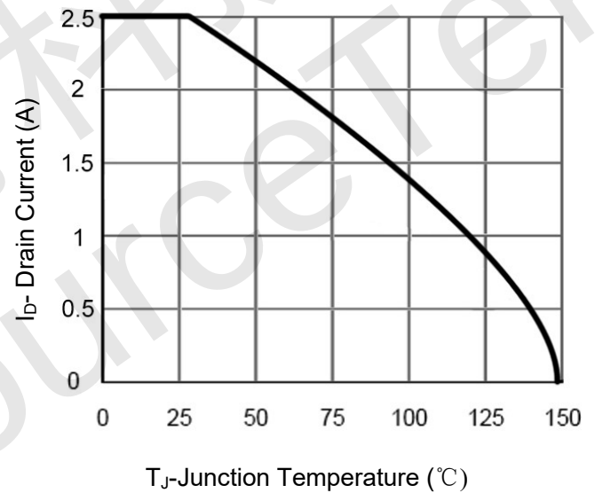
Figure 4 Drain Current
