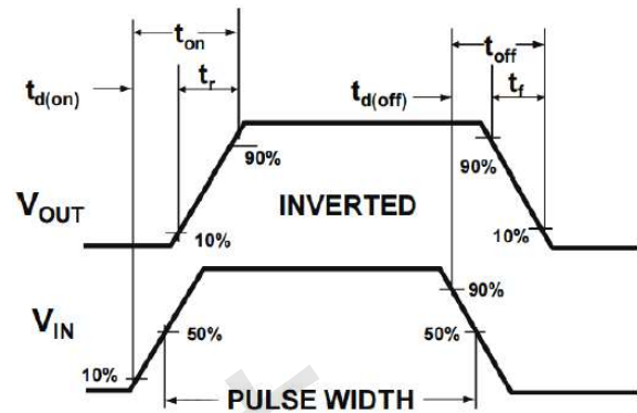
Figure 2 Switching Waveform
