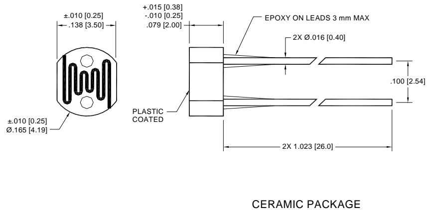
PACKAGE DIMENSIONS INCH [mm]
