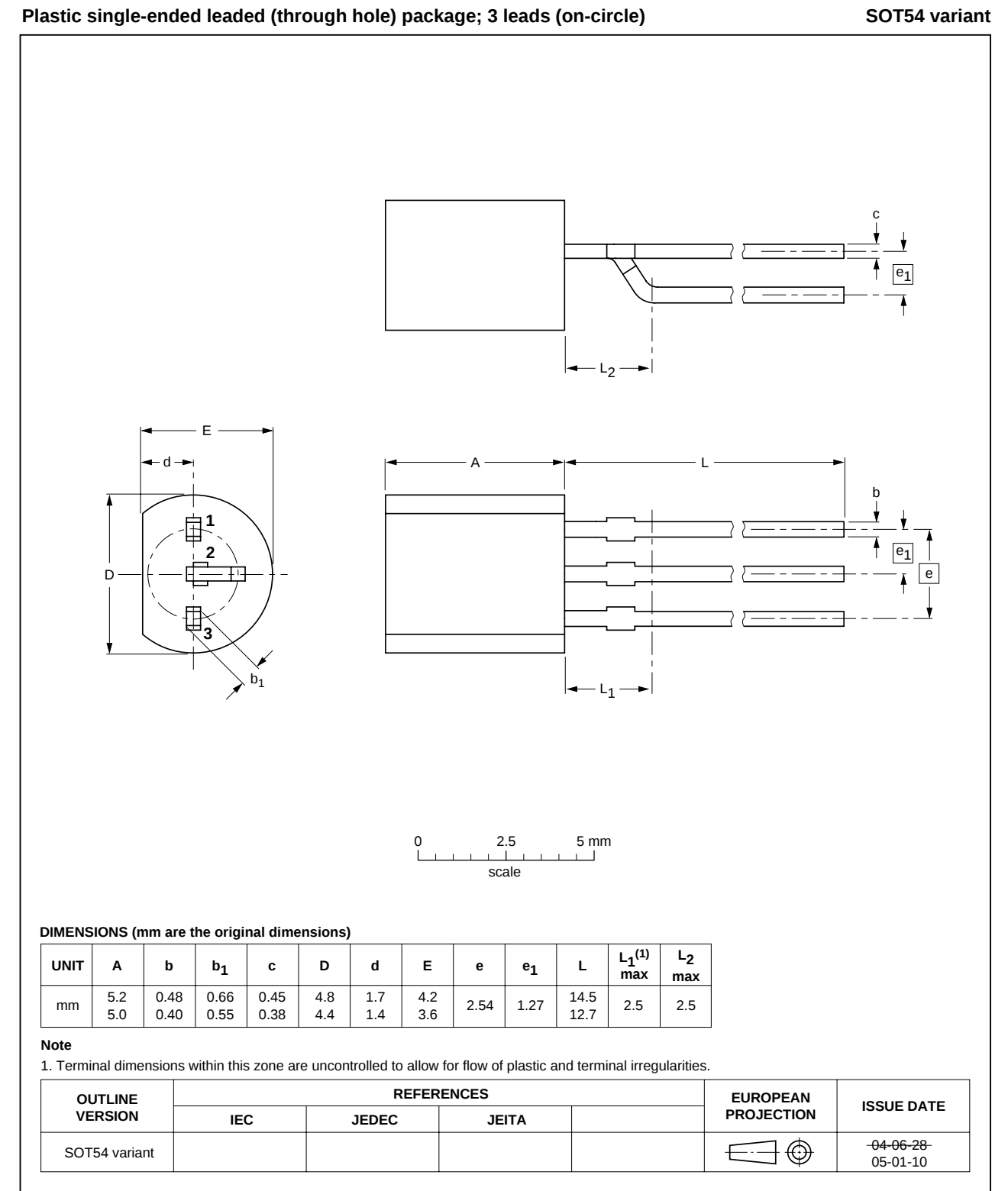
Fig 10. Package outline SOT54 variant
