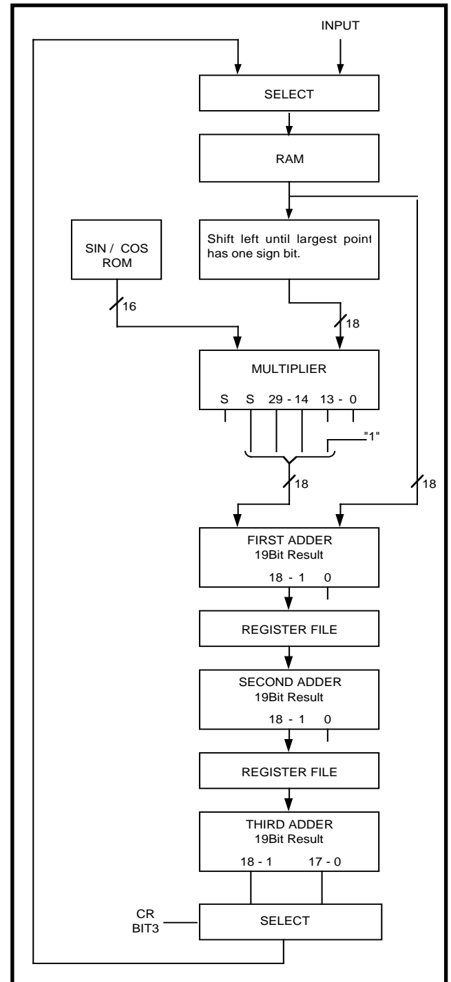
Figure 3 One of Four Data Paths
