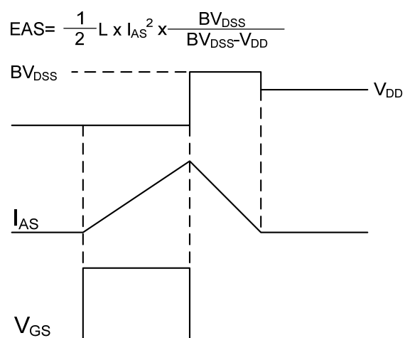
Fig.8 EAS Waveform
