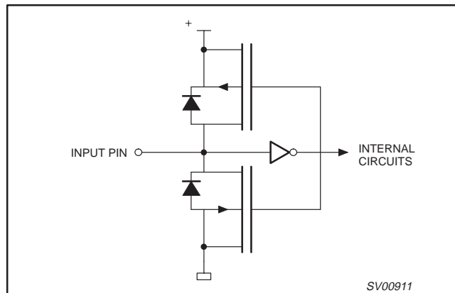
Figure 2. Bushold circuit
