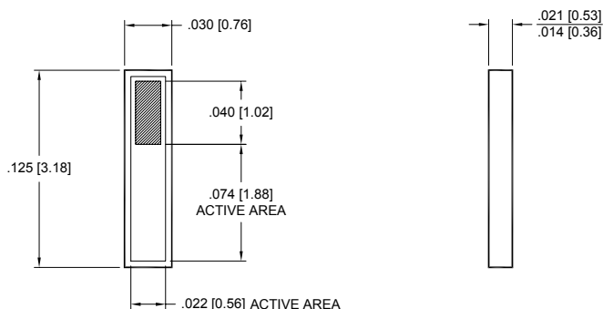
SOLDERABLE PHOTODIODE
