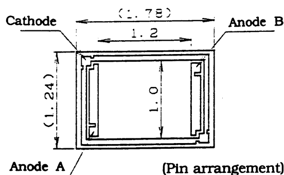
[ Chip drawing (20/1) ]
