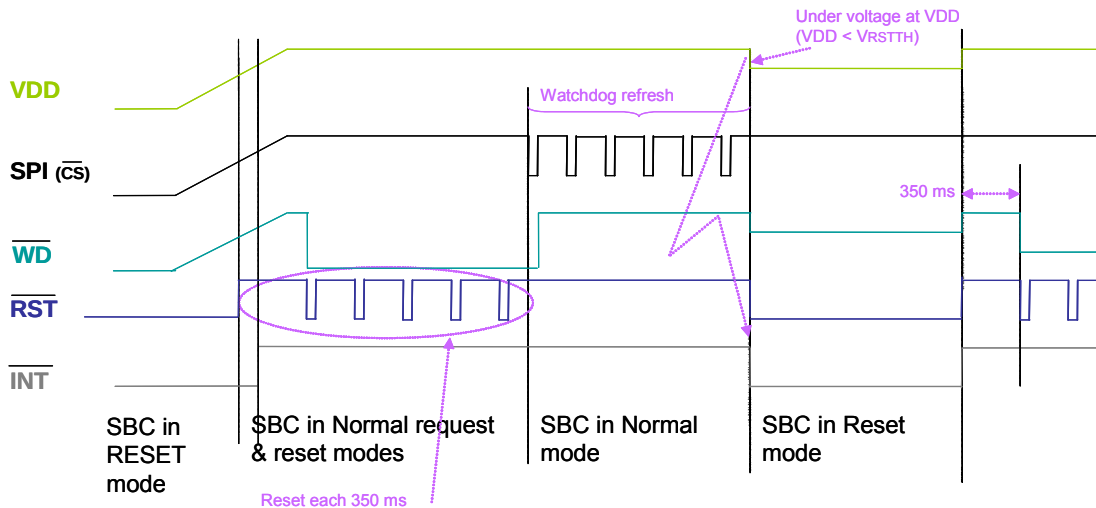
Figure 34. Undervoltage on VDD
