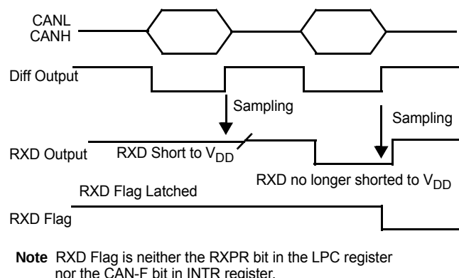
Figure 26. RXD Recovery Conditions
