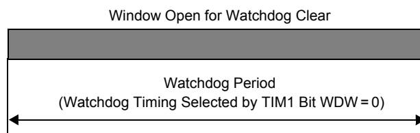
Figure 29. Timeout Watchdog
