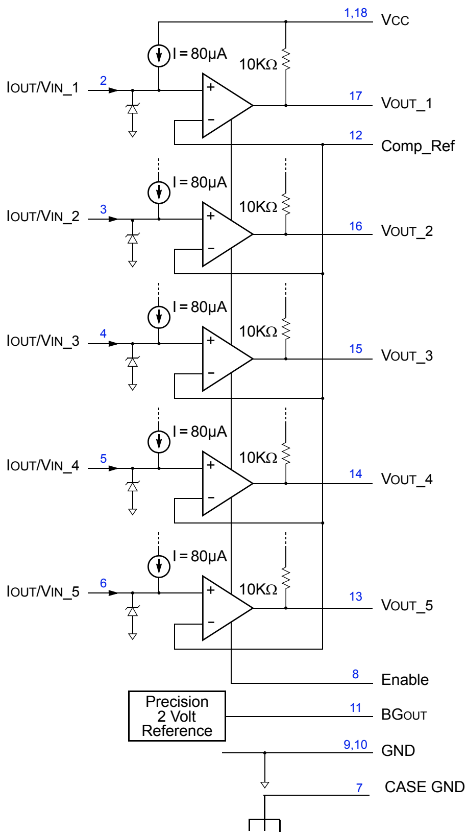
FIGURE 1 – Schematic Diagram
