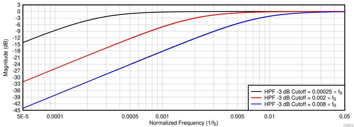
Figure 42. HPF Filter Frequency Response Plot
