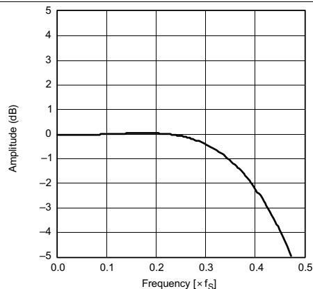
Transition characteristics
