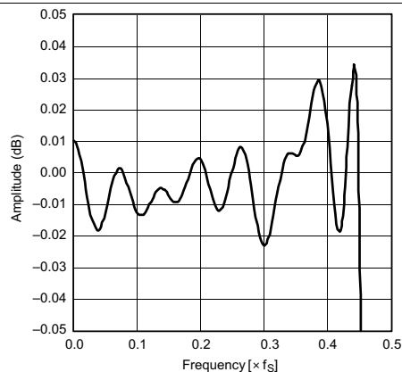
Pass-band ripple
