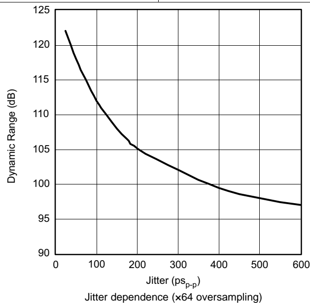
Figure 37. Dynamic Range vs Jitter
