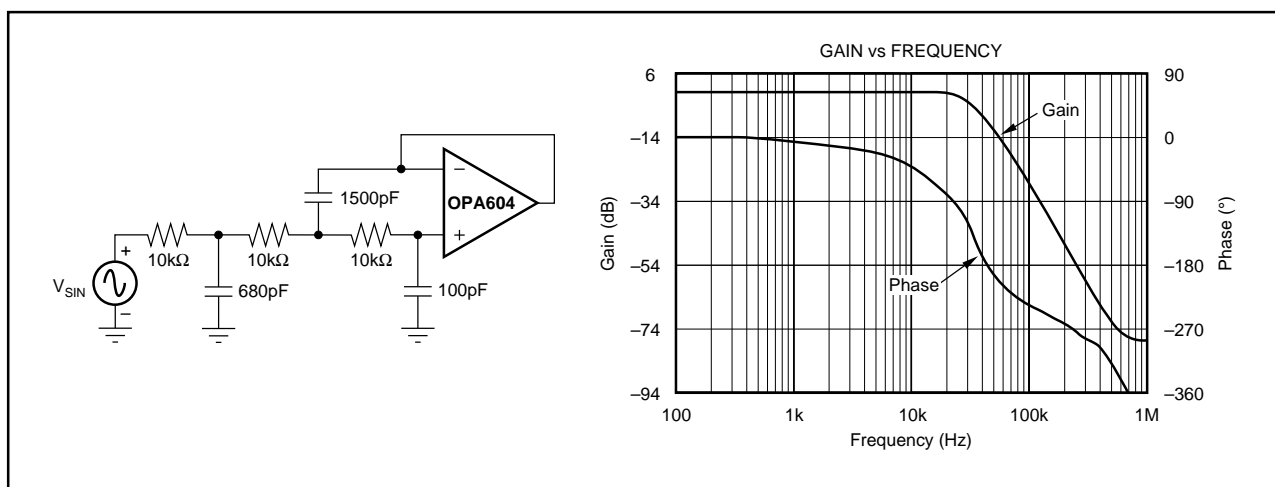
FIGURE 11. 3rd-Order LPF.
