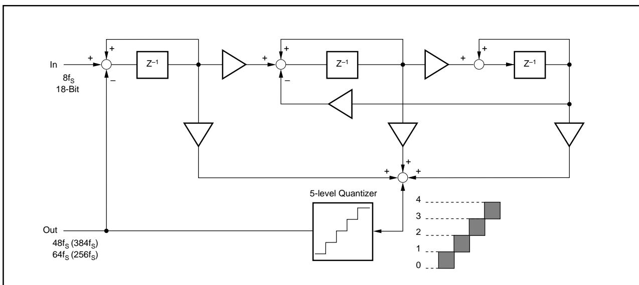
FIGURE 15. 5-Level \Delta\Sigma Modulator Block Diagram.
