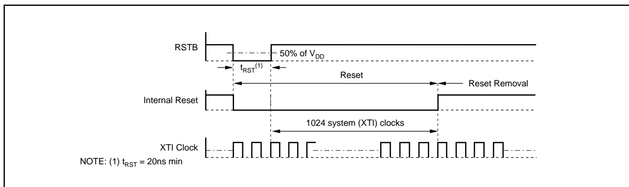
FIGURE 13. RSTB-Pin Reset Timing.
