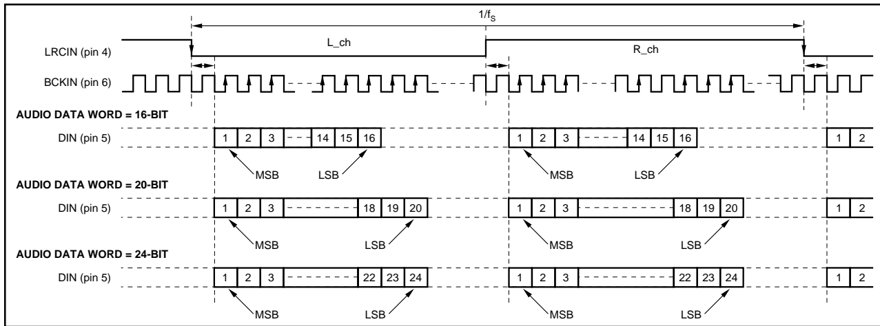
FIGURE 5. "I2S" Data Input Timing.
