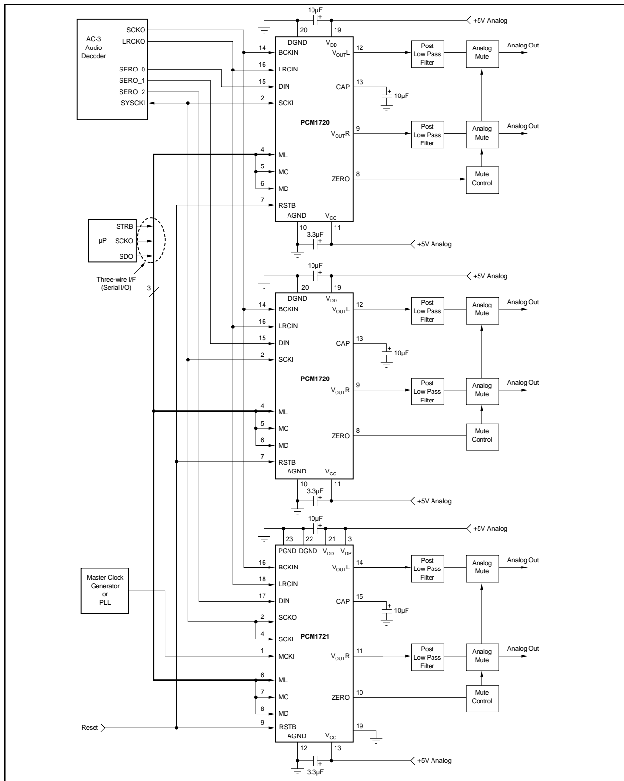
FIGURE 17. Connection Diagram for a 6-Channel AC-3 Application.
