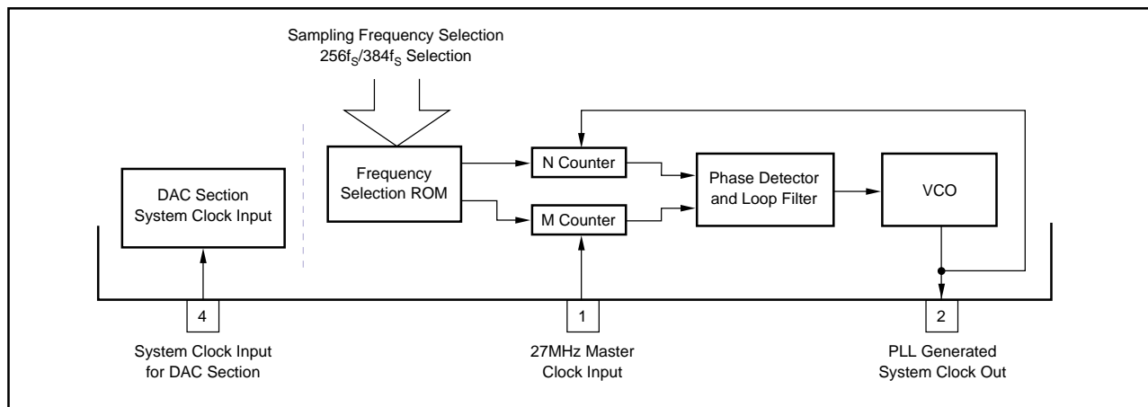
FIGURE 2. PPL Block Diagram.
