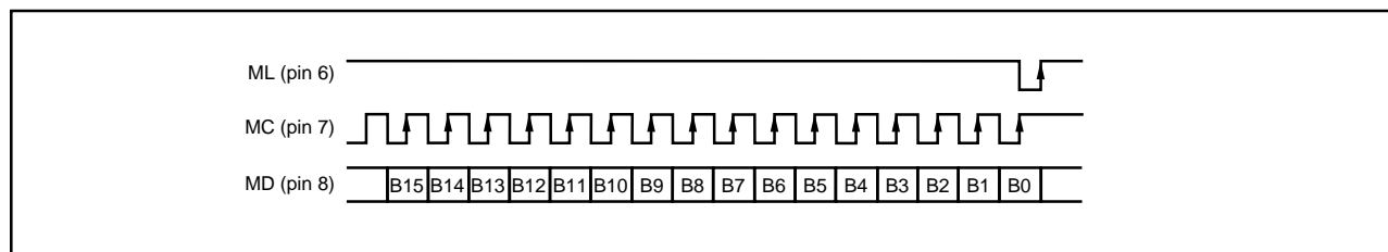
FIGURE 7. Serial Interface Timing.
