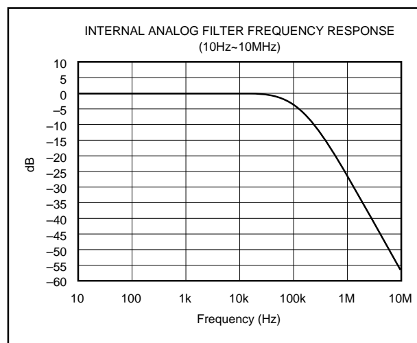
FIGURE 10. Low Pass Filter Wideband Frequency Response.
