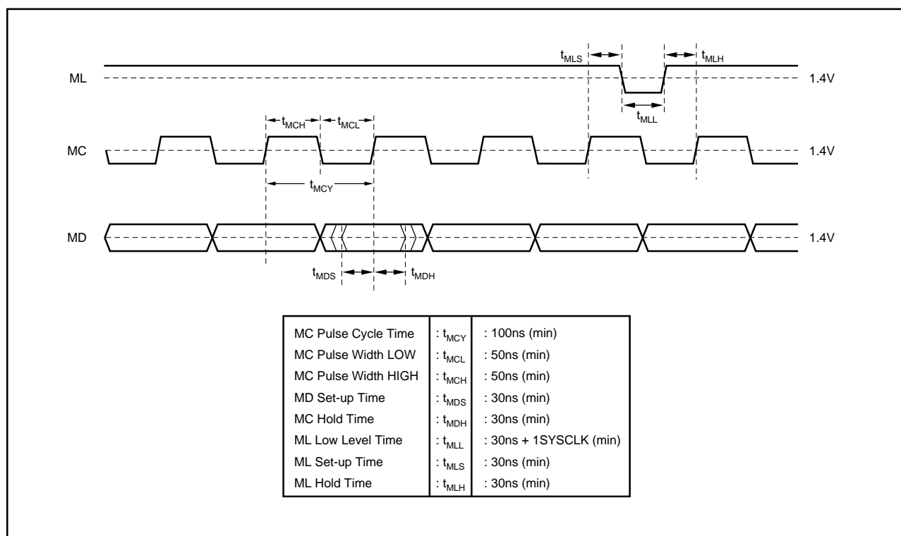
FIGURE 8. Program Register Input Timing.
