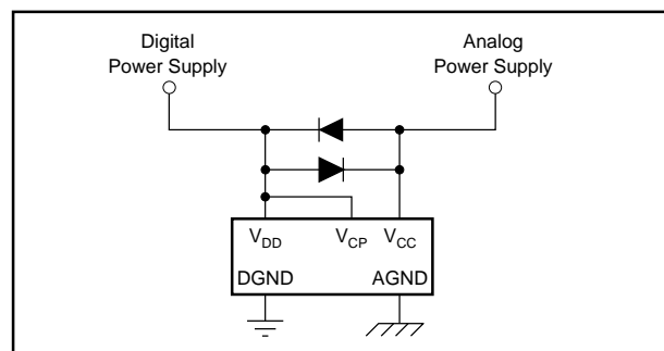
FIGURE 14. Latch-up Prevention Circuit.
