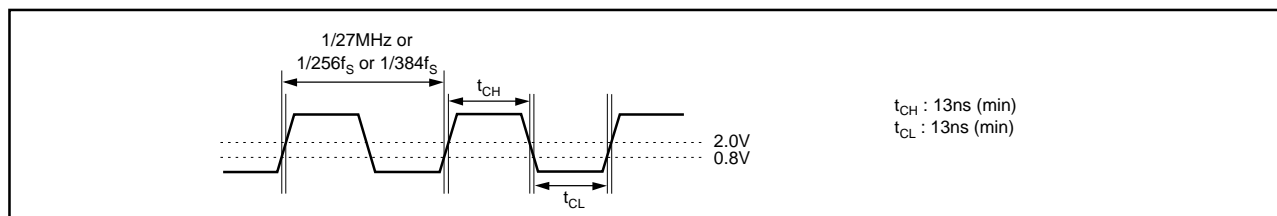
FIGURE 3. MCKI, SCKI Input Timing.
