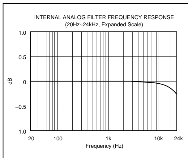
FIGURE 9. Low Pass Filter Frequency Response.
