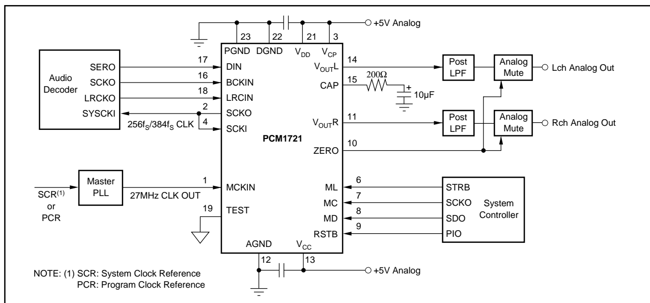
FIGURE 1. External Master Clock Input.
