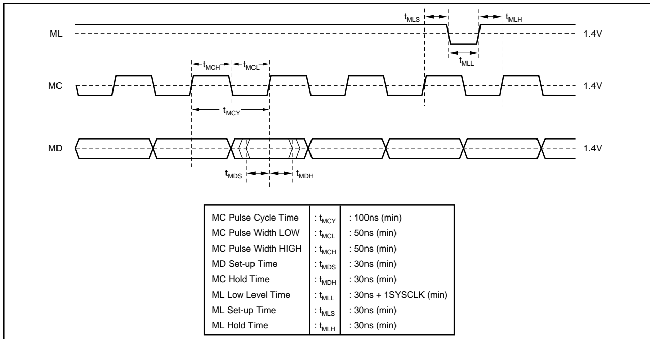
FIGURE 6. Serial Interface Timing.
