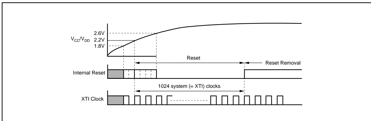
FIGURE 12. Internal Power-On Reset Timing.
