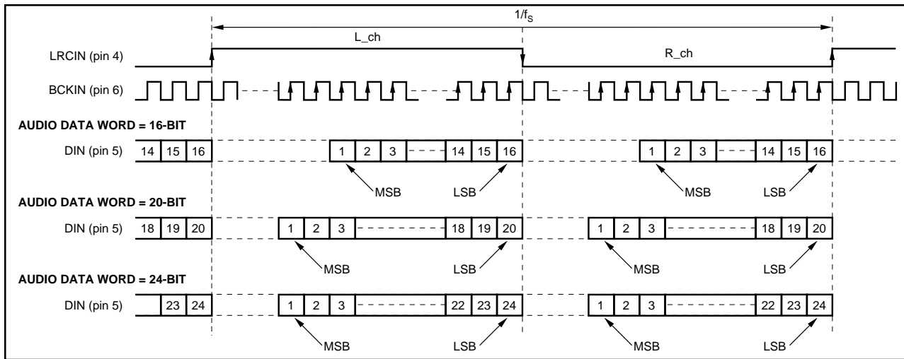
FIGURE 4. "Normal" Data Input Timing.
