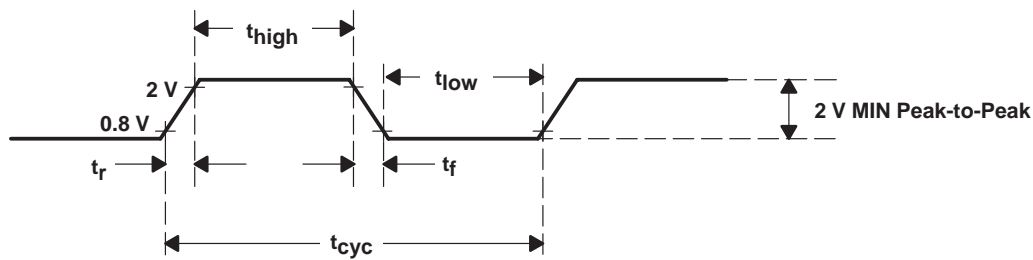
Figure 26. PCLK Timing Waveform
