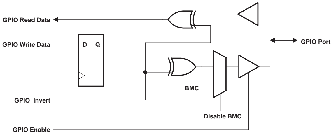
Figure 22. BMC/LINKON/GPIO0
