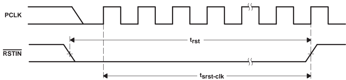
Figure 27. \overline{\text{RSTIN}} Timing Waveforms
