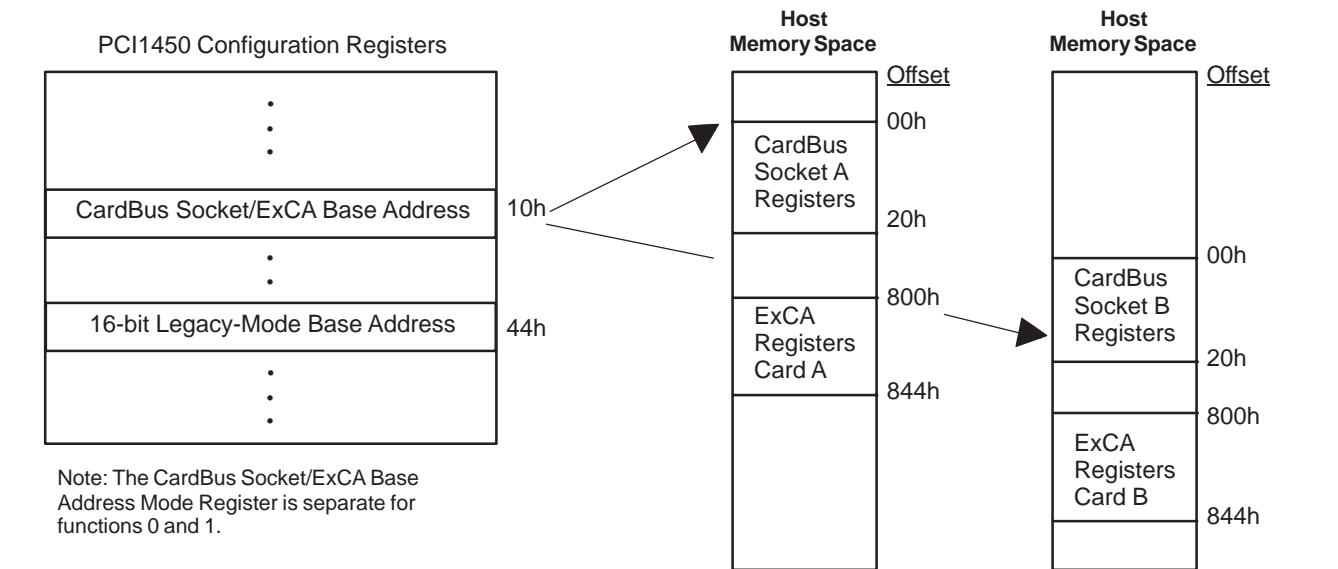
Figure 21. Accessing CardBus Socket Registers Through PCI Memory
