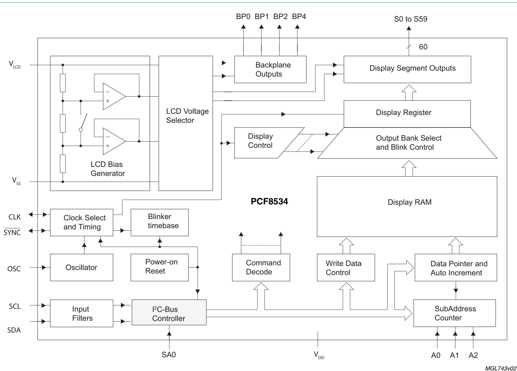
Fig 1. PCF8534 block diagram
