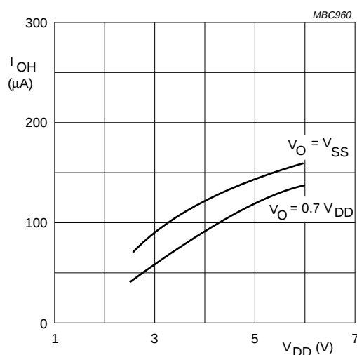
Fig.10 Typical HIGH level pull-up output source current ( I_{OH} ) as a function of operating supply voltage ( V_{DD} ).
