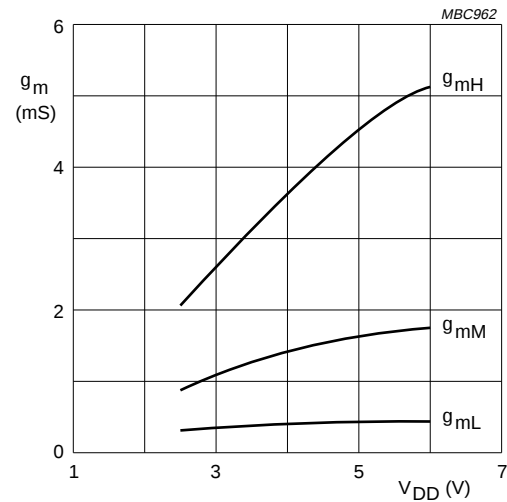
Fig.12 Typical transconductance values ( g_m ) as a function of operating supply voltage ( V_{DD} ) for the options g_{mL} , g_{mM} and g_{mH} .
