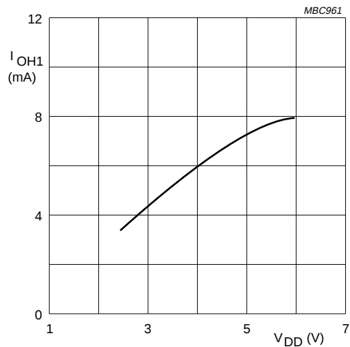
Fig.11 Typical HIGH level push-pull output source current ( I_{OH1} ) as a function of operating supply voltage ( V_{DD} ).
