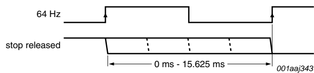
Fig 32. STOP bit release timing
