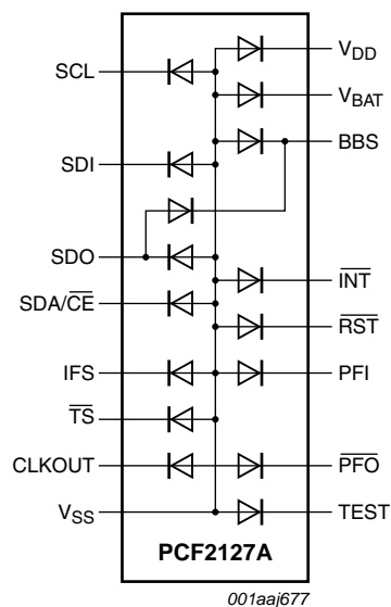
Fig 46. Device diode protection diagram of PCF2127A
