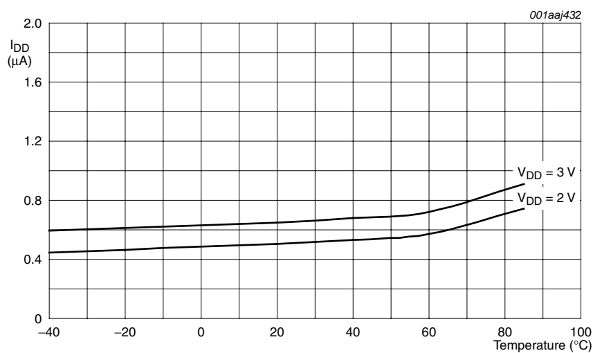
Fig 48. I DD as a function of temperature
