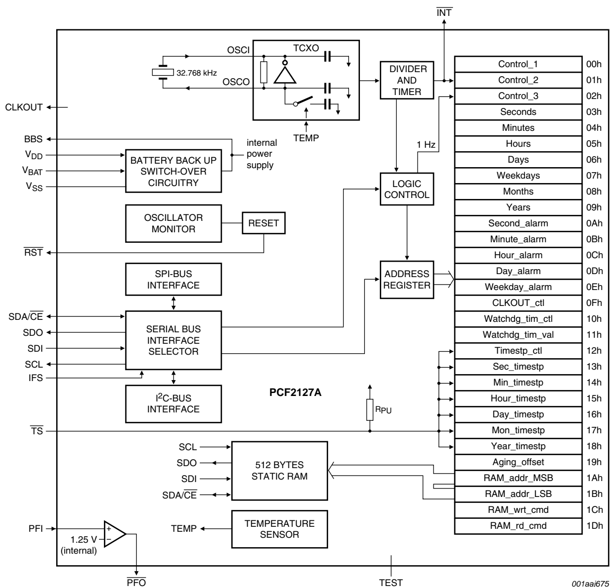
Fig 1. Block diagram of PCF2127A
