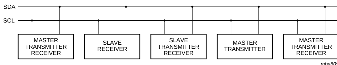
Fig 15. System configuration
