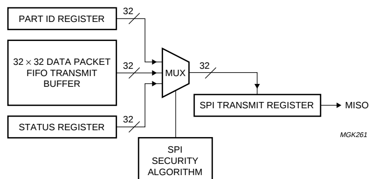
Fig.9 SPI transmit functional block diagram.
