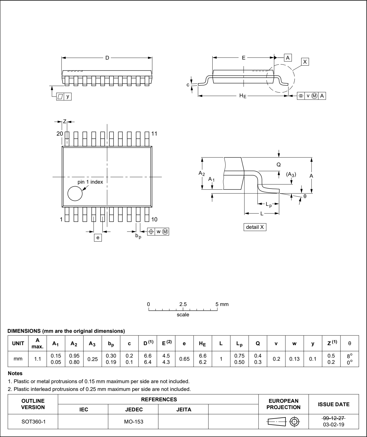
Figure 21. Package outline SOT360-1 (TSSOP20)
