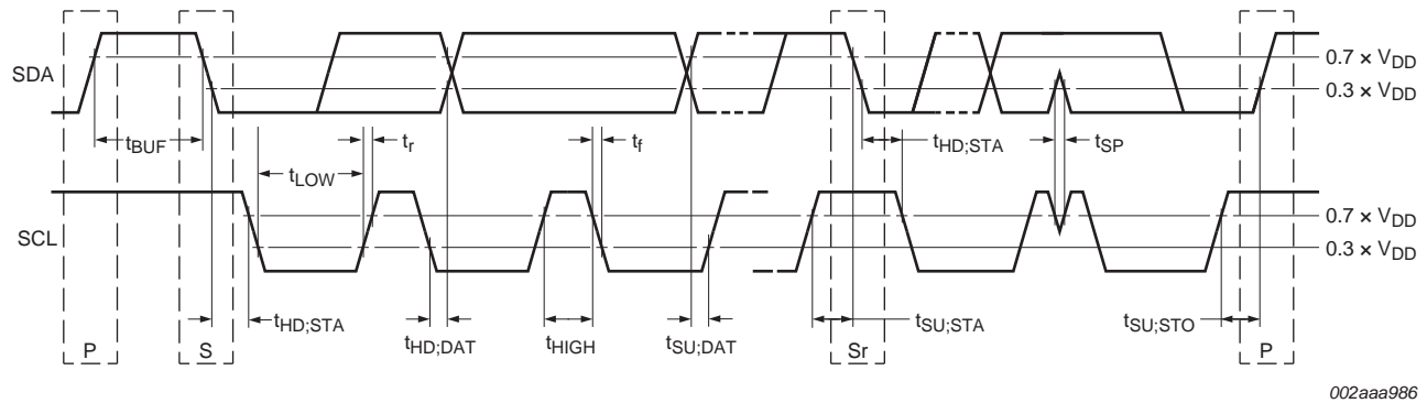
Fig 14. Definition of timing
