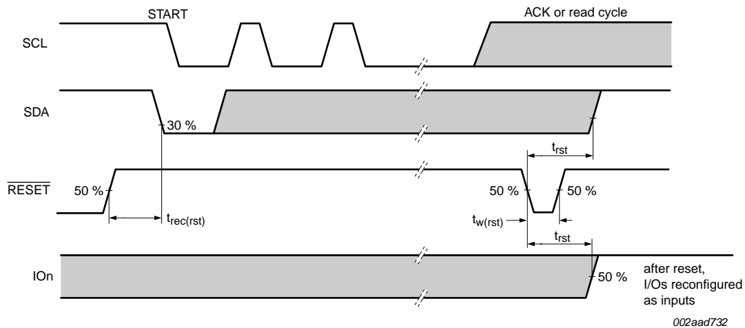
Fig 16. Definition of RESET timing
