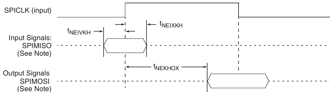
Figure 3-23. SPI AC Timing in Slave Mode (External Clock) Diagram
