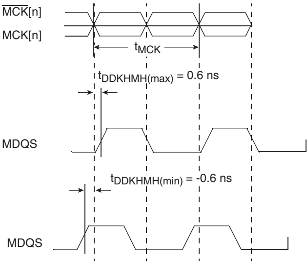
Figure 3-4. Timing Diagram for t_{DDKMH}
