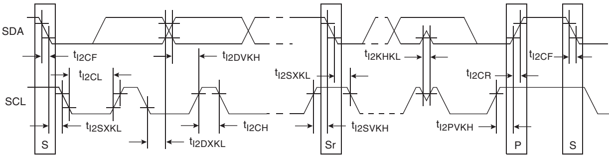
Figure 3-15. I 2 C Bus AC Timing Diagram
