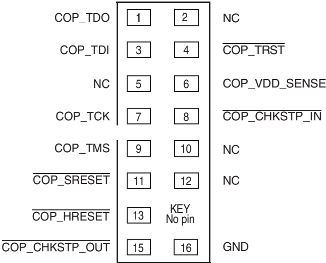
Figure 4-5. COP Connector Physical Pinout
