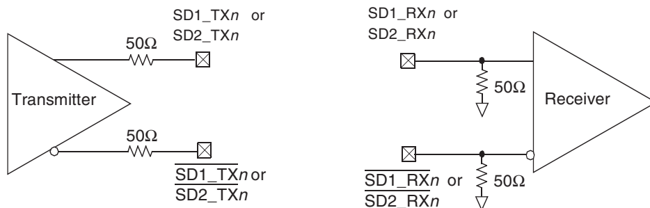
Figure 3-39. SerDes Transmitter and Receiver Reference Circuits
