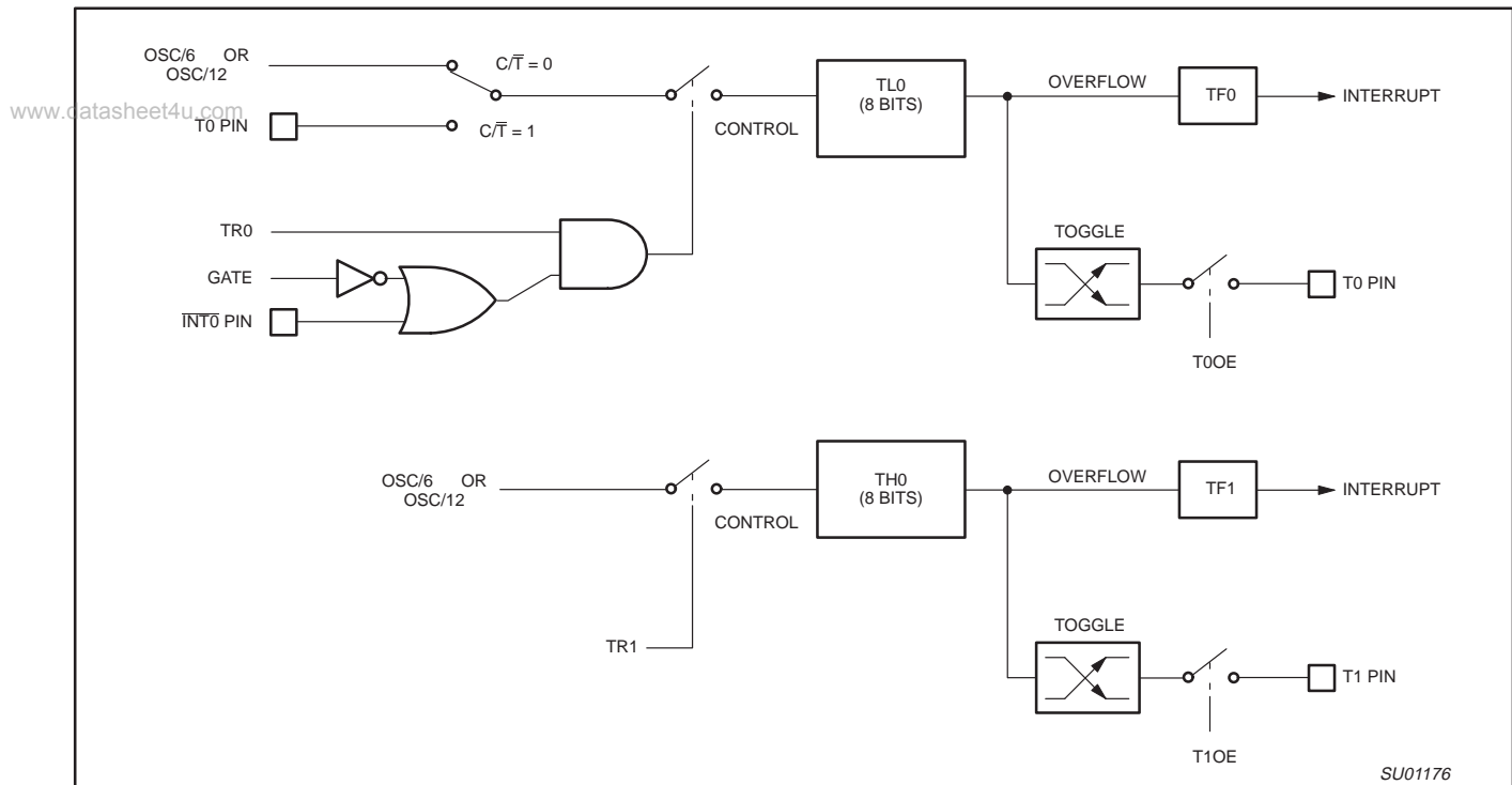
Figure 27. Timer/Counter 0 Mode 3 (Two 8-Bit Counters)
