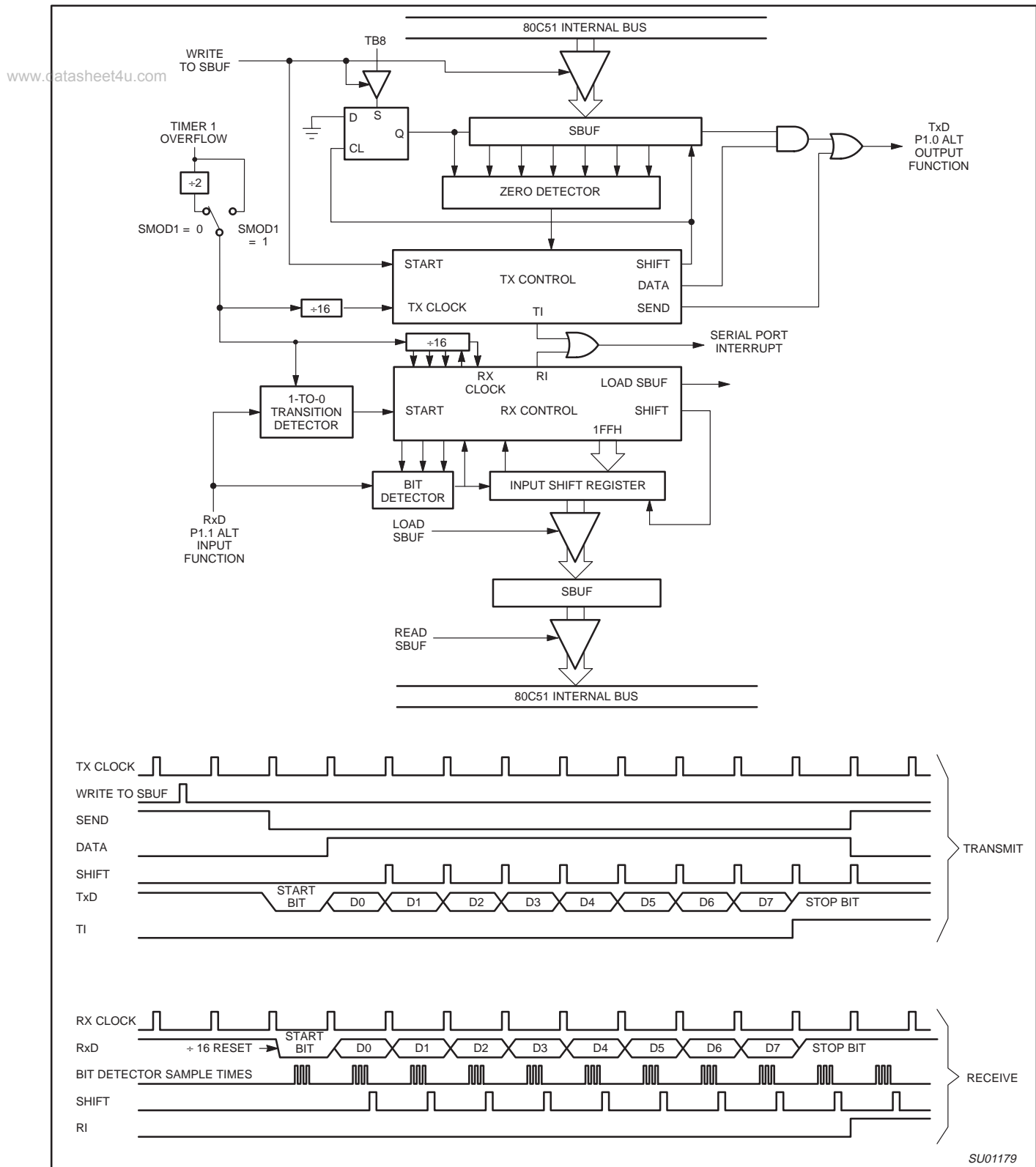
Figure 30. Serial Port Mode 1
