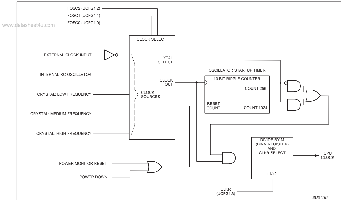
Figure 18. Block Diagram of Oscillator Control
