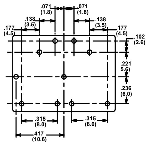
Bottom View PC Board Layout
