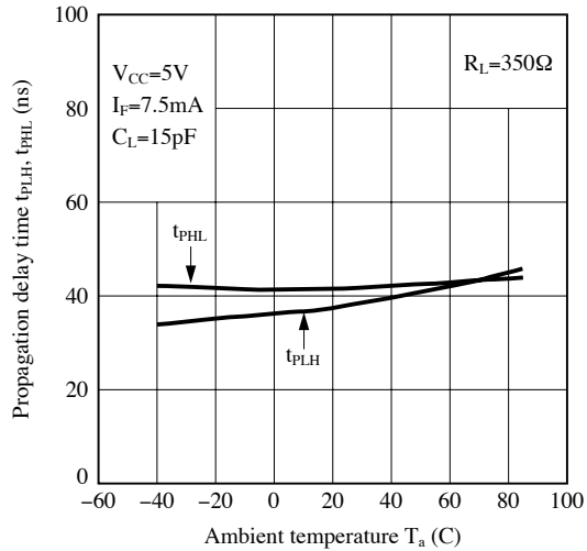
Fig.11-c Propagation Delay Time vs. Ambient Temperature
