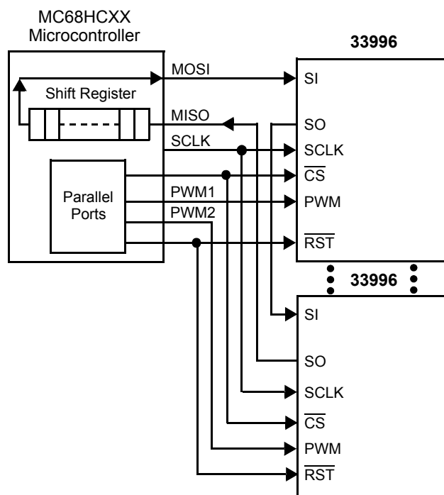
Figure 4. 33996 SPI System Daisy Chain
