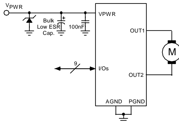
Figure 12. Avalanche Protection
