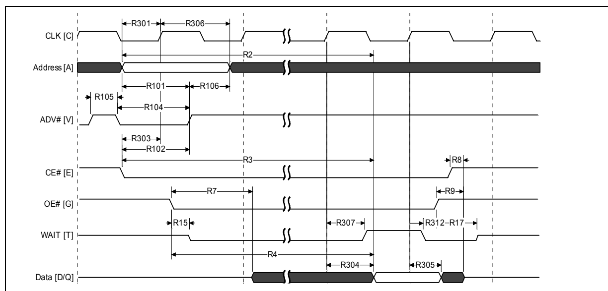
Figure 17: Synchronous Single-Word Array or Non-array Read Timing
