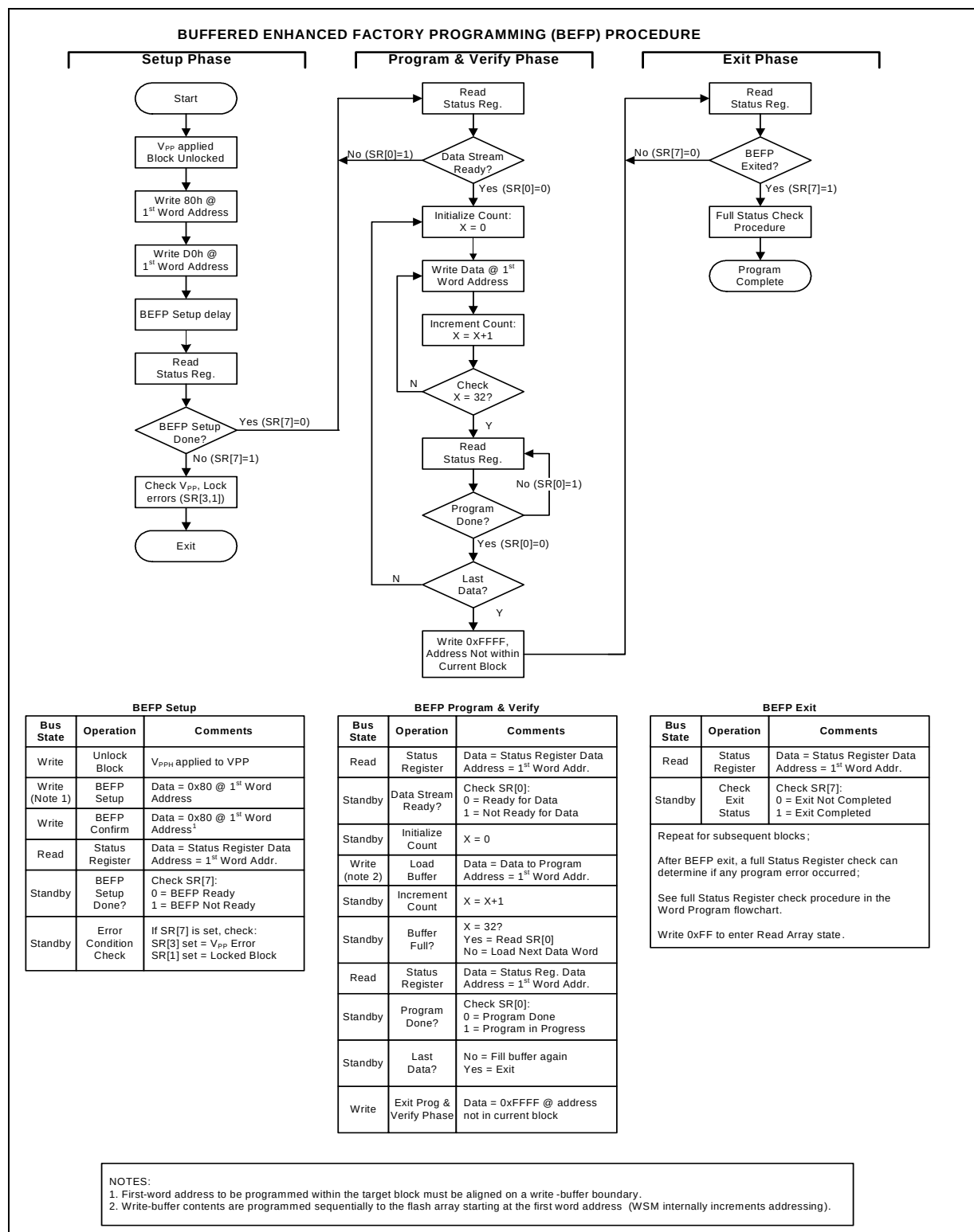
Figure 43. BEFP Flowchart
