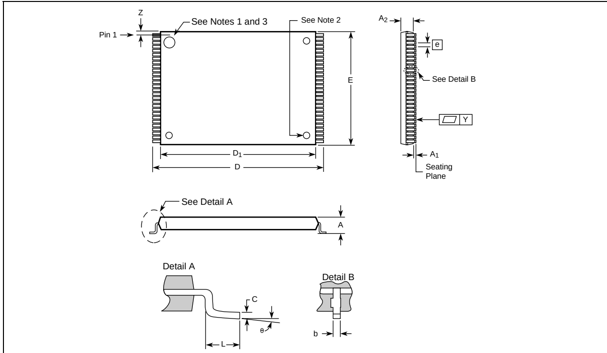
Figure 3. 56-Lead TSOP Package Drawing and Specifications
