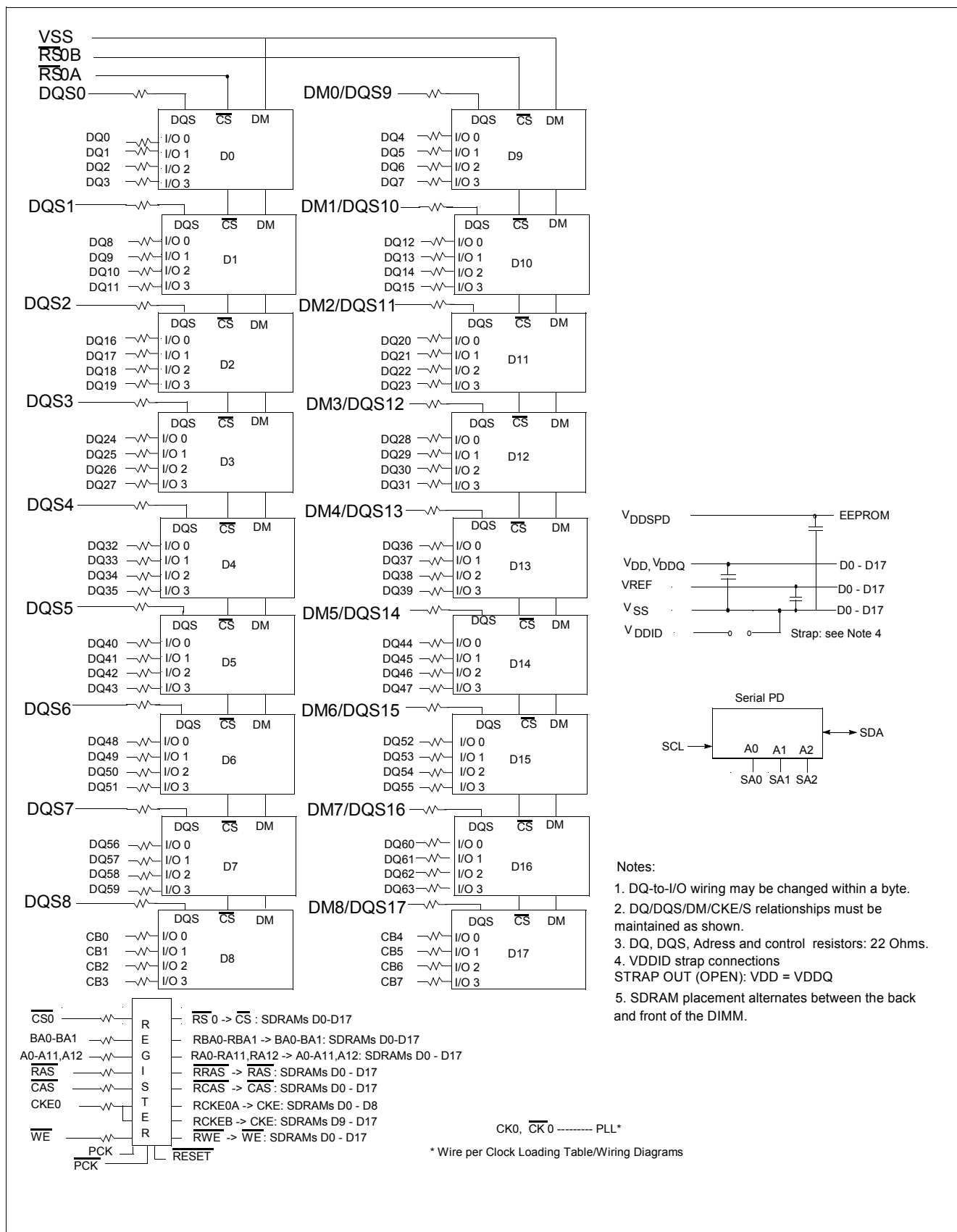
Figure 4 Block Diagram: One Rank 64M × 72 DDR-I SDRAM DIMM Modules (64M×4 components) HYS72D64300GBR on Raw Card C
