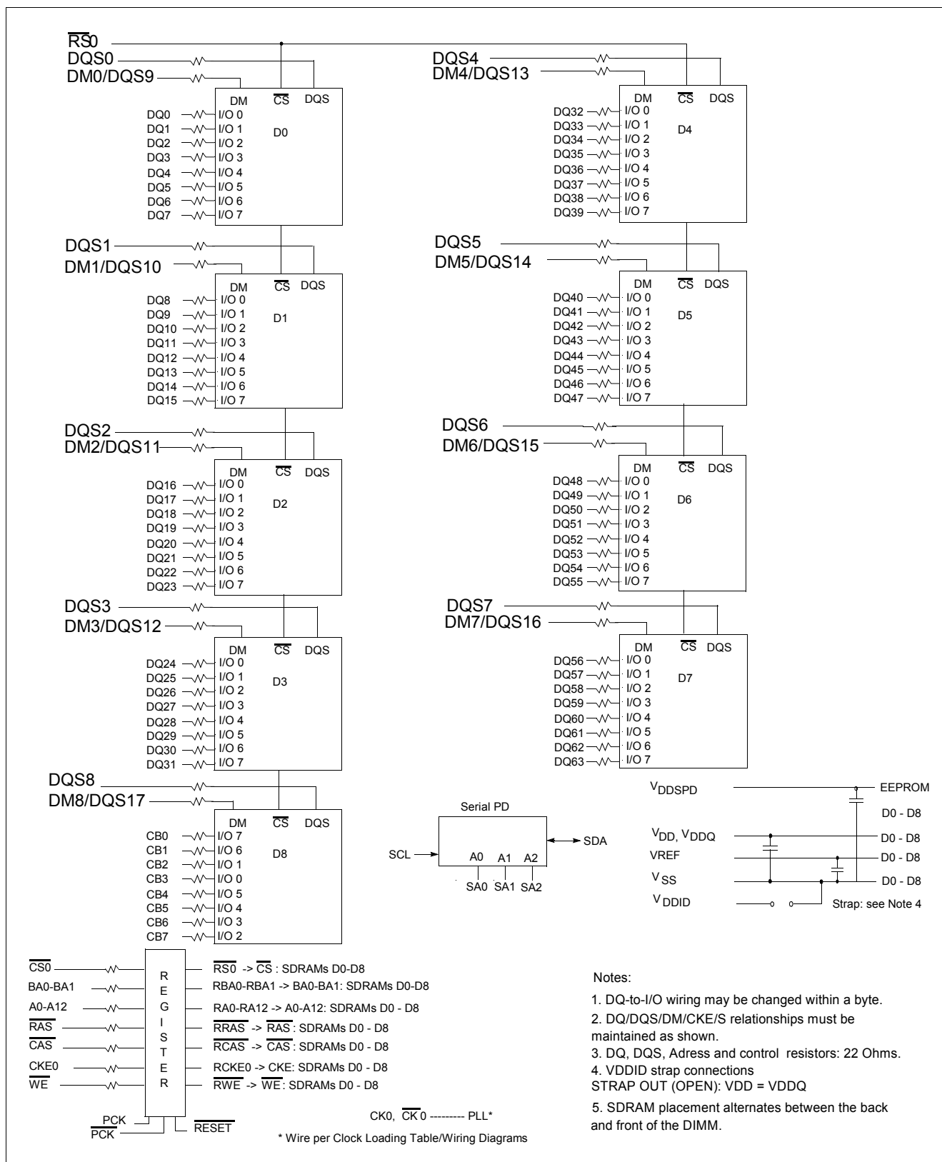
Figure 2 Block Diagram: One Rank 32M × 72 DDR SDRAM DIMM Module (32M×8 components) HYS72D32300GBR on Raw Card A
