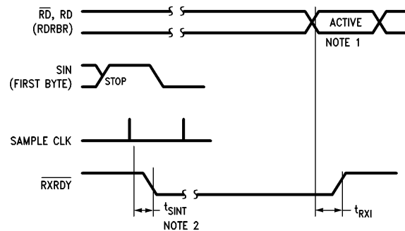
Figure 11. Receiver Ready (Pin 29) FCR0 = 0 or FCR0 = 1 and FCR3 = 0 (Mode 0)
